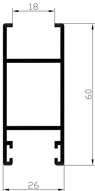
Hoja lateral H=18 mm Ref: 9216
