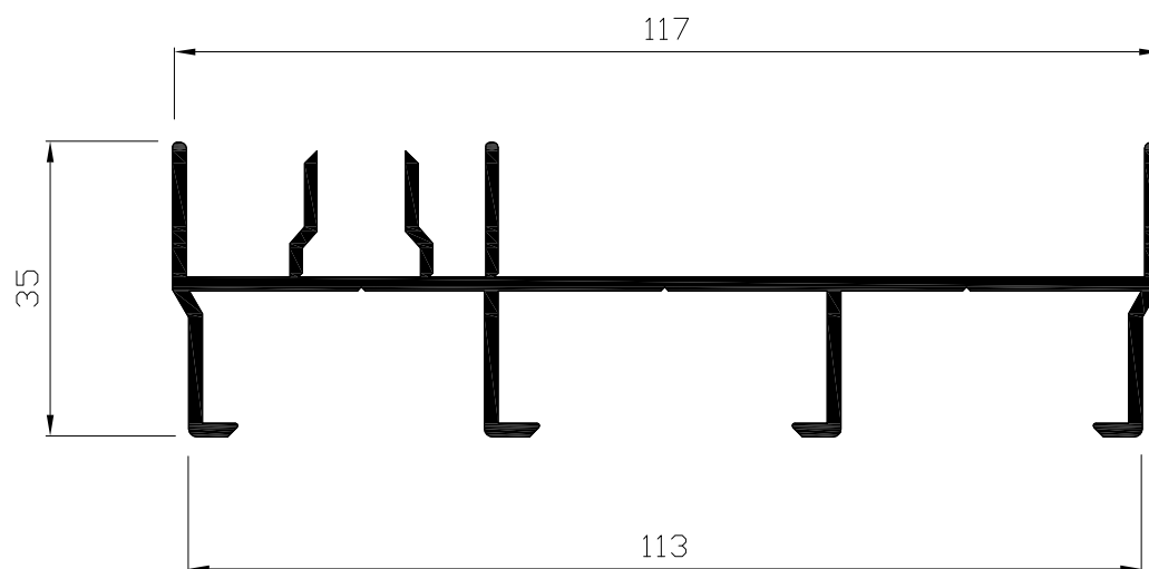
Marco lateral 3 carriles
