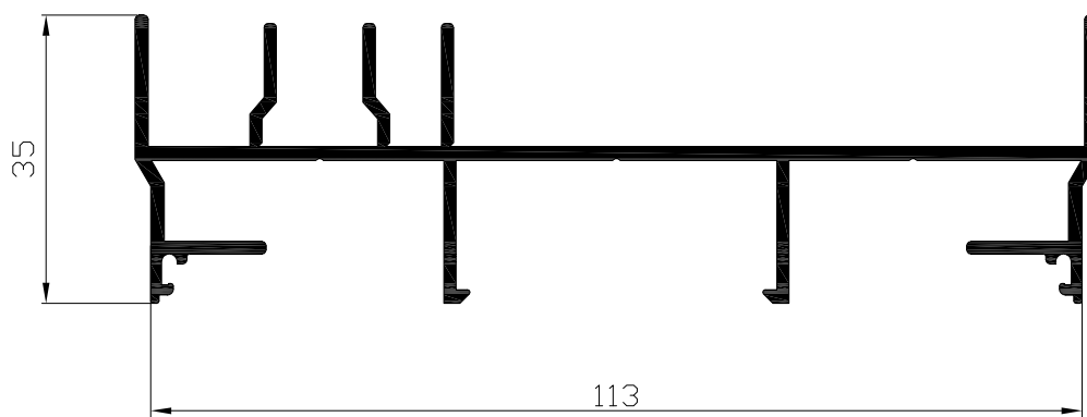
Marco lateral curvo Ref: 8213
