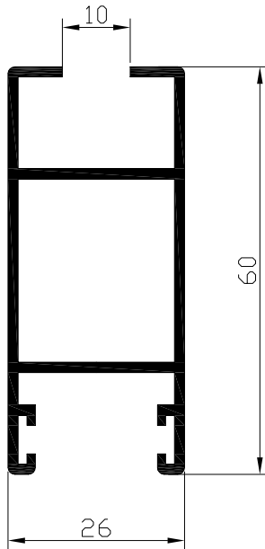
Hoja lateral H=10 mm Ref: 9206
