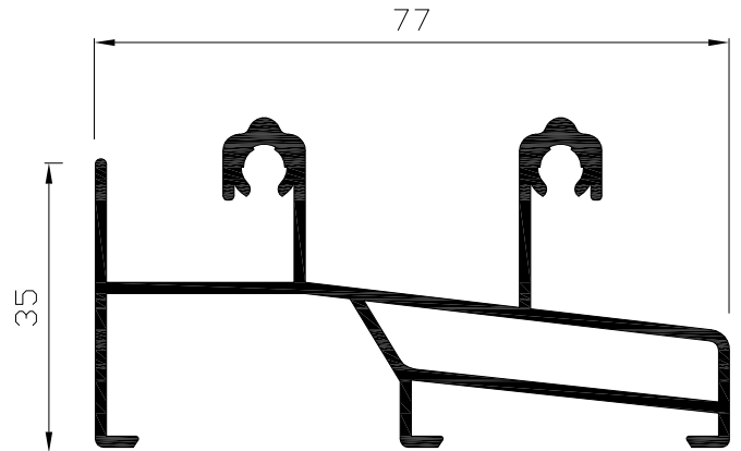
Marco inferior Ref: 9202
