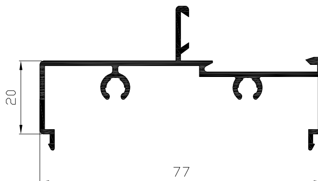
Marco lateral Ref: 8203
