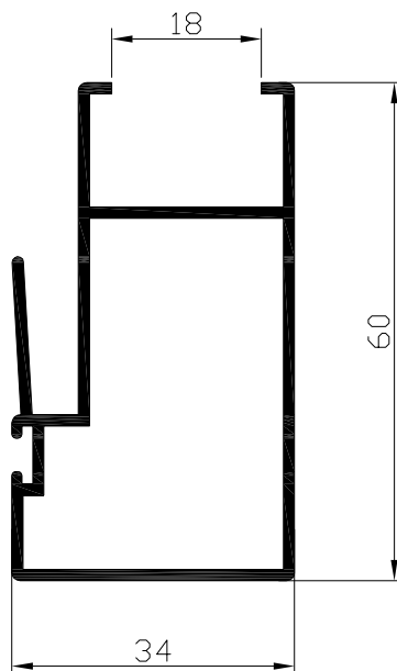
Hoja central H=18 mm Ref: 9215
