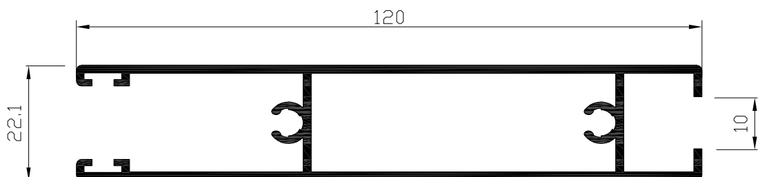
Zócalo H=10 mm Ref: 9207
