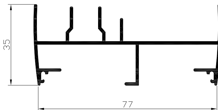
Marco lateral curvo Ref: 8213
