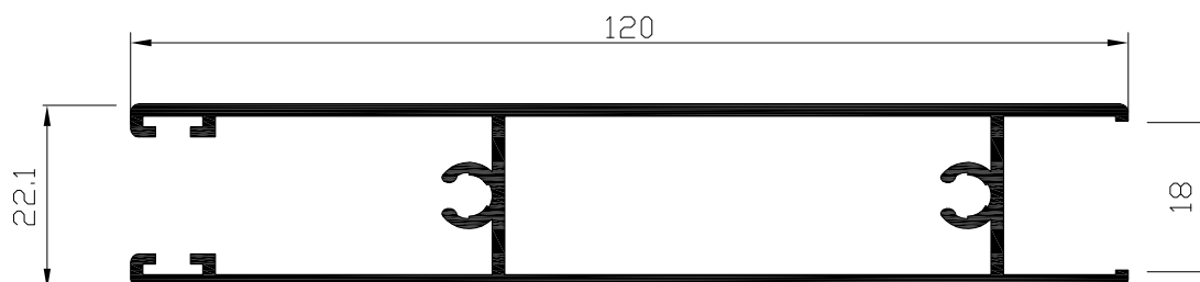
Zócalo H=18 mm Ref: 9217
