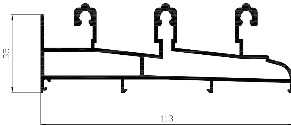
Marco lateral 3 carriles Ref: 8233
