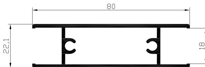
Parteluces H=18 mm Ref: 9218
