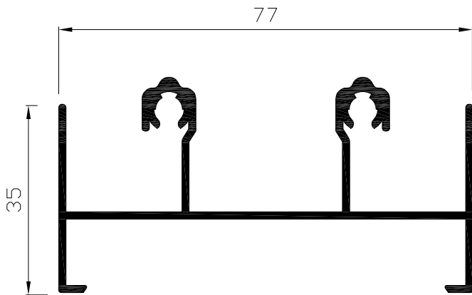
Marco superior Ref: 9201
