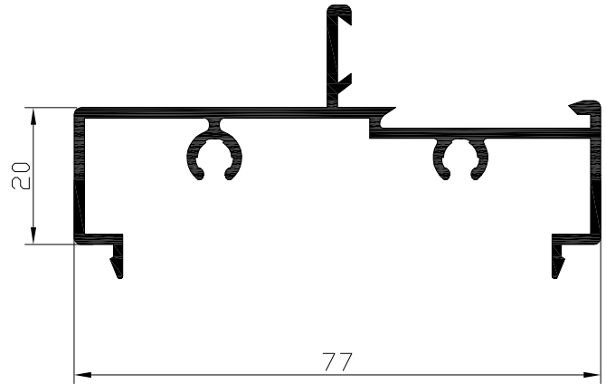
Marco lateral Ref: 9203
