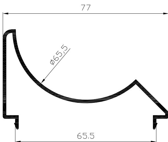
Esquinero graduable Ref: 9321
