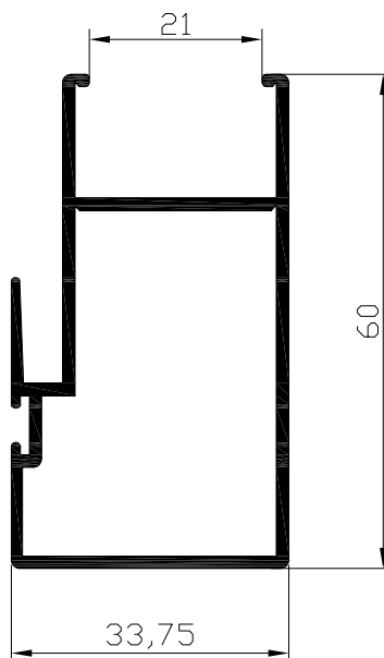
Hoja central H=21 mm Ref: 9235
