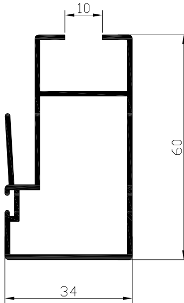
Hoja central H=10 mm Ref: 9205
